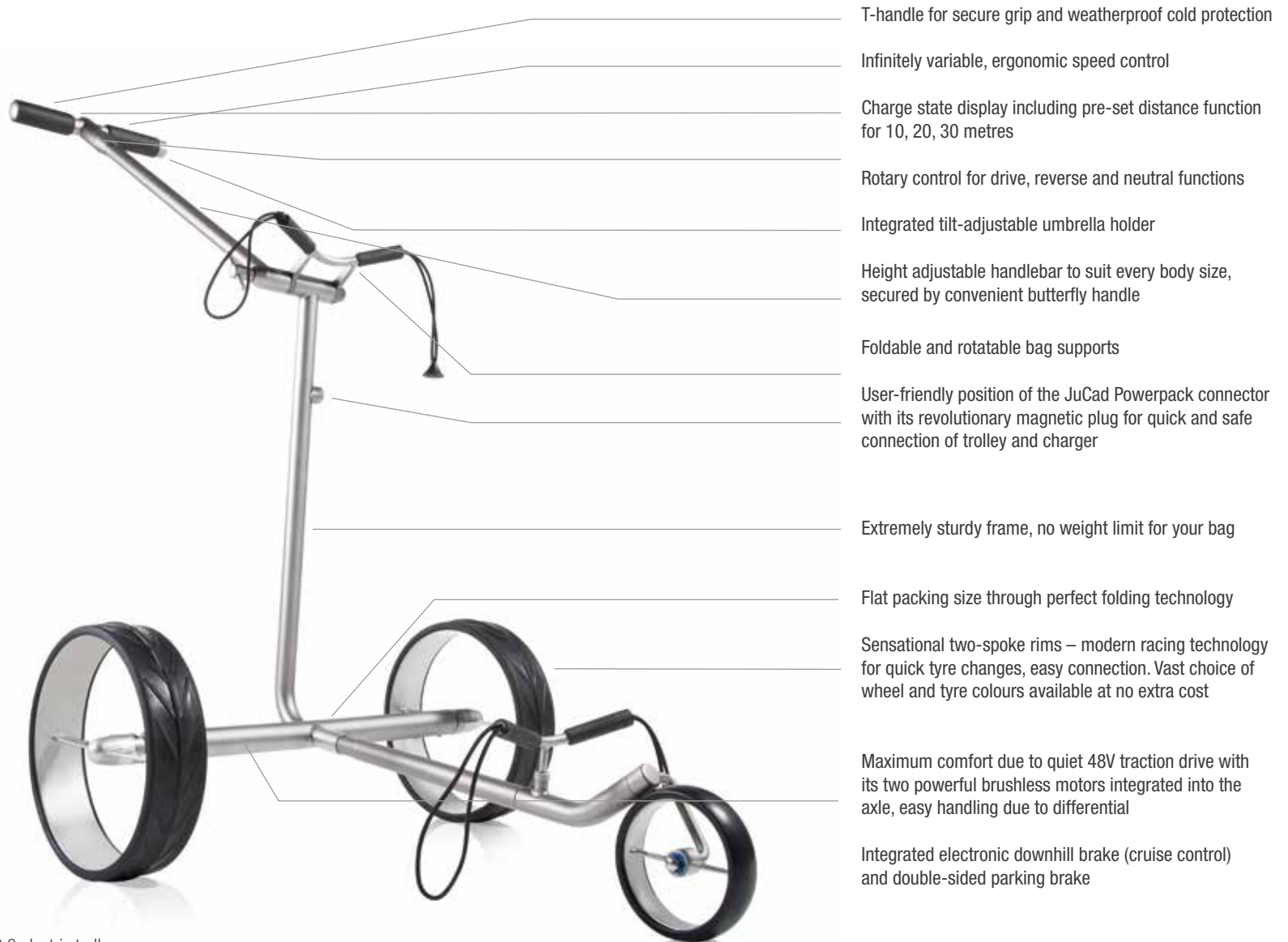
JuCad Ghost Titan 2.0 electric trolley
